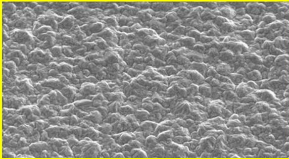
12µm untreated-side Foil SEM × 1500
