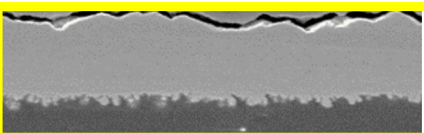
12µm Foil Cross Section × 1000
